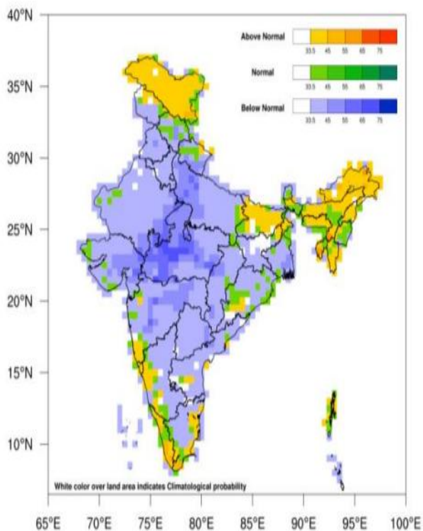
Maximum Temperature Outlook for July 2025
