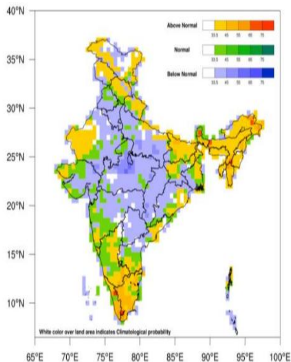
Minimum Temperature Outlook for July 2025
